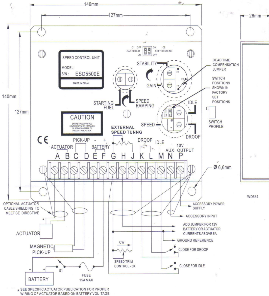
DIAGRAM 1. ESD5500E Series Wiring Diagram and Outline
